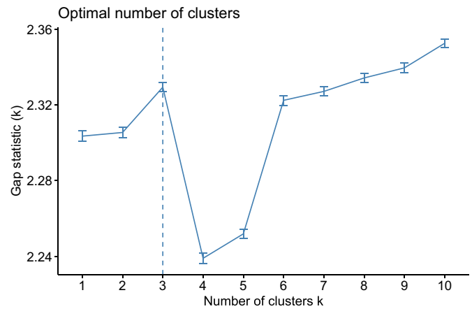
Fig. 2. The optimal number of clusters computed by the gap statistic. Three clusters is found to be the optimal number.
